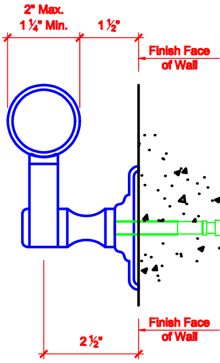
Hidden Anchor Bolt
