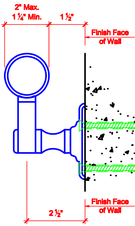
Exposed Flat Head Screw
